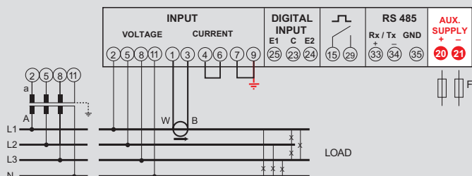
3-phase network, 4 wire, 1 System
