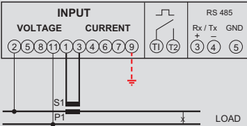
Single phase network
