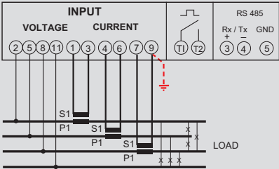
3-phase network, 4 wire
