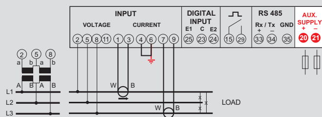
3-phase network, 3 wire (ARON L1-L3)
