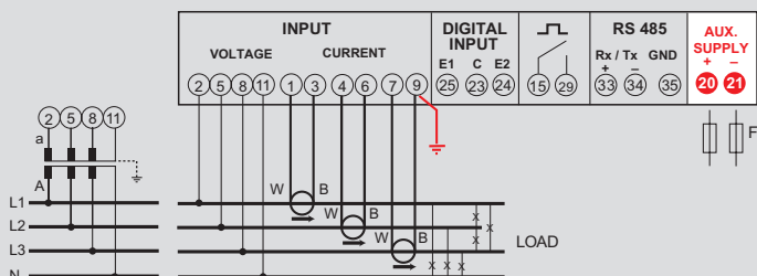
3-phase network, 4 wire
